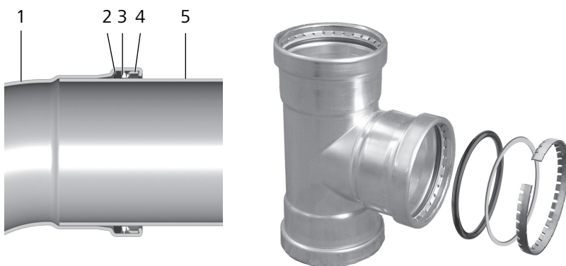
(1) Fitting, (2) Dichtring, (3) Trennring, (4) Schneidring, (5) Rohr
